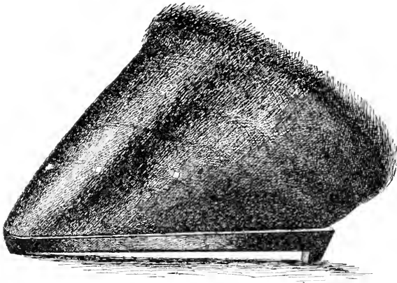
FIG. 15.—Side view of a fore hoof shoe so as to quicken the "breaking over" (quicken the action) in a "forger." Note the short shoe, heel calks inclined forward, and the rolled toe.
